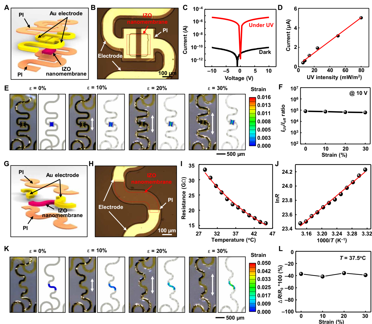
Fig. 3. Characteristics of UV and temperature sensors. (A) Schematic exploded view of the IZO nanomembrane-based UV sensor. (B) Optical microscopic image of the UV sensor. (C) I-V characteristics of the UV sensor. (D) Calibration curve of the IZO UV sensor. (E) Sequential images of the UV sensor under strain and corresponding FEA results of IZO. (F) I_{UV}/I_{dark} for UV light under strain. (G) Schematic exploded view of the IZO temperature sensor. (H) Optical microscopic image of the temperature sensor. (I) Calibration curve of the temperature sensor. (J) Plot of \ln R versus 1000/T of the temperature sensor. (K) Sequential images of the IZO temperature sensor under strain and corresponding FEA results of IZO. (L) Relative resistance change of the temperature sensor under strain.
